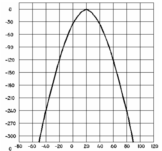
TUNING FORK CRYSTAL TEMPERATURE CURVE
